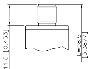
Z - 4 pole connector M12x1
