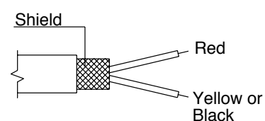
Cable gland with shielded cable 2x0.25 - 1m.
