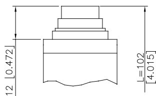
Z - 4 pole connector M12x1
