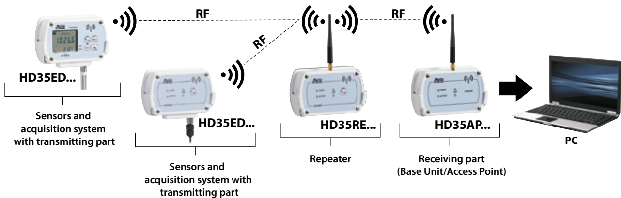
Wireless data recording system with repeater
