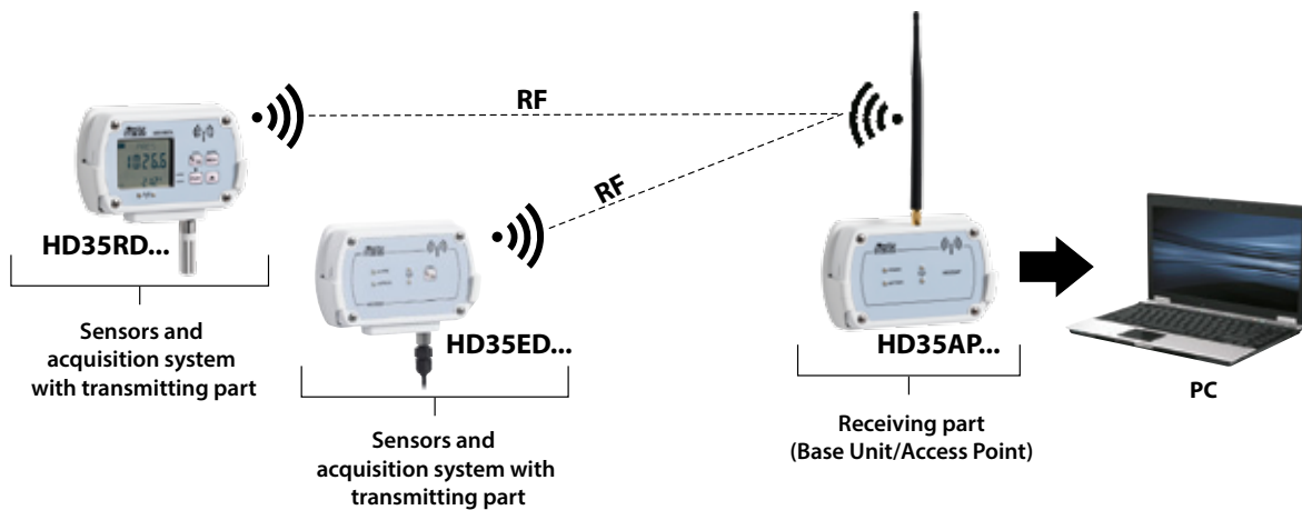
Delta OHM wireless data recording system
