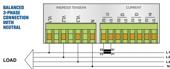
BALANCED 3-PHASE CONNECTION MULTIPLE LOADS
